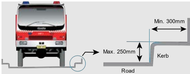
Figure 16. Carriageway kerb clearance dimensions.
